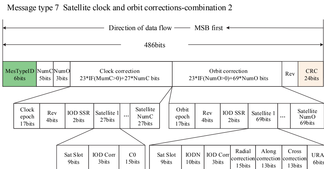
Figure 6-9 Format layout of message type 7
